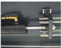
带防爆阀的油缸。 Oil cylinder with explosion-proof valve.
