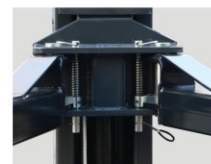
加强型滑台内置锁 Strengthen carriage Inner arm lock
